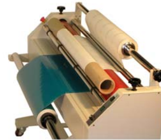
Lamination Reel & Passive Take-up
